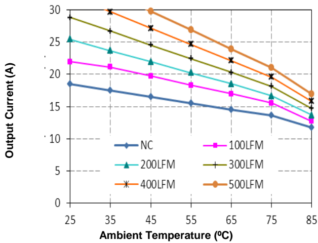
Figure 9. Current Derating Curve for Airflow Direction 3 (Ref. Fig. 10 for Airflow Direction; typical Vin, open frame unit, solder interface)
