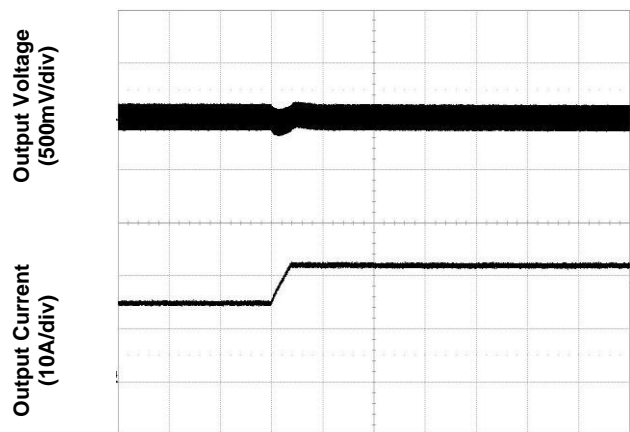
Figure 6. Transient Load Response (typical Vin, load current steps from 50% to 75% at a slew rate 0.1A/µs, 1,000µF external output capacitance)
