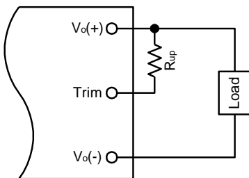
Figure 16. Circuit to Increase Output Voltage
